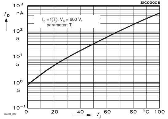
Figure 8. Typical Off-State Current
