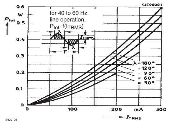
Figure 9. Power Dissipation
