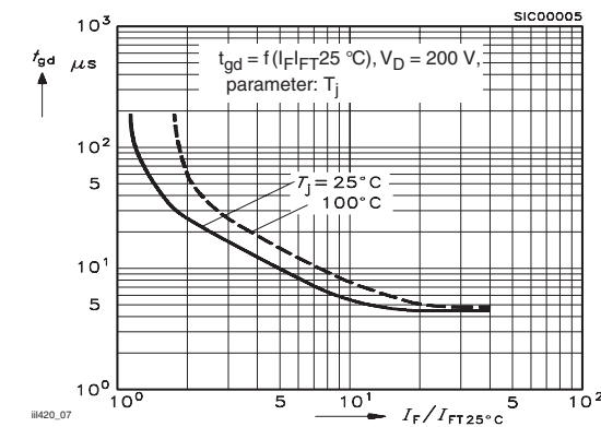
Figure 7. Typical Trigger Delay Time
