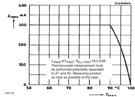
Figure 6. Current Reduction
