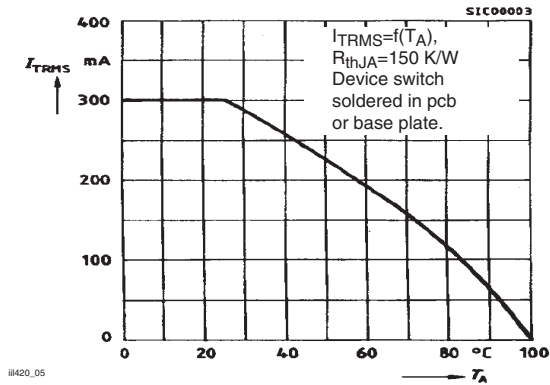
Figure 5. Current Reduction
