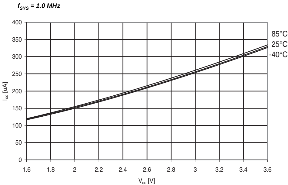
Figure 35-4. Active Supply Current vs. V_{\text{CC}}
