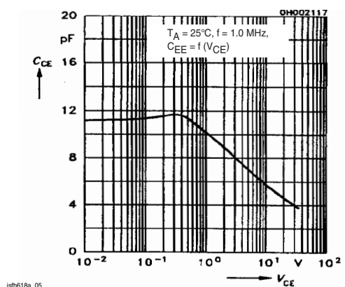
Figure 7. Transistor Capacitance
