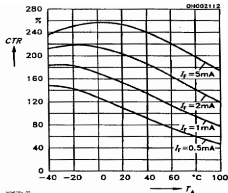
Figure 4. Current Transfer Ratio (typ.)
