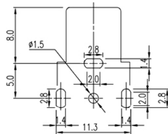
T:1.6 Dimensions of PC board holes Tolerance : \pm 0.05 (Printed-bottom view)
