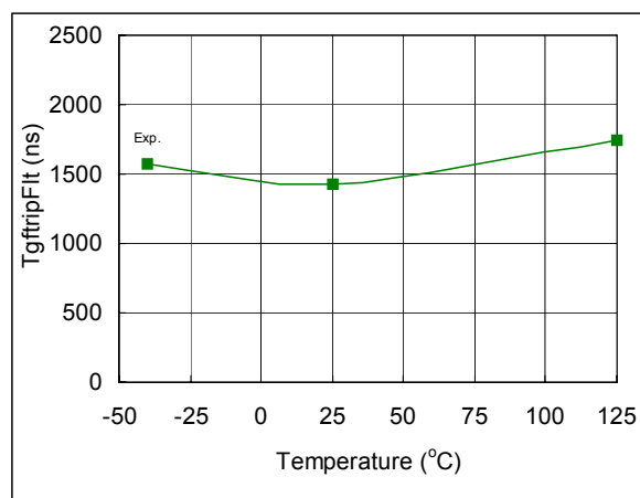
Fig. 77. GF TRIP to Fault Time vs. Temperature
