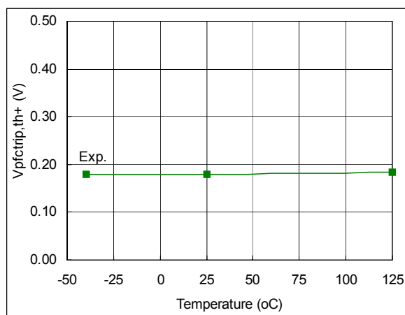
Fig. 100. PFC Positive Going Threshold vs. Temperature
