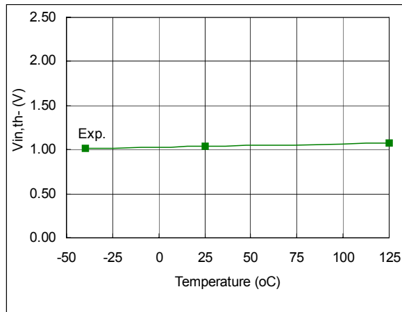
Fig. 95. Input Negative Going Threshold vs. Temperature
