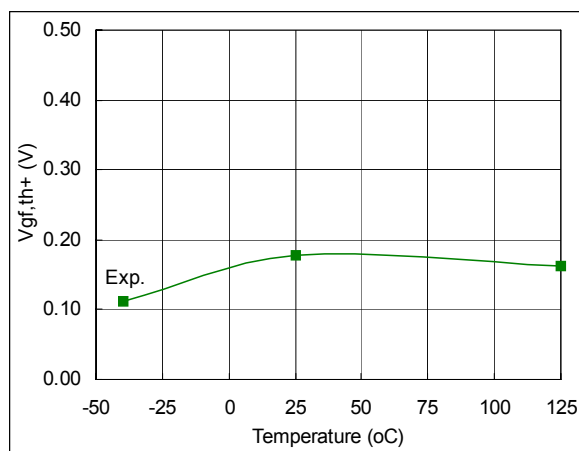
Fig. 102. GF Positive Going Threshold vs. Temperature
