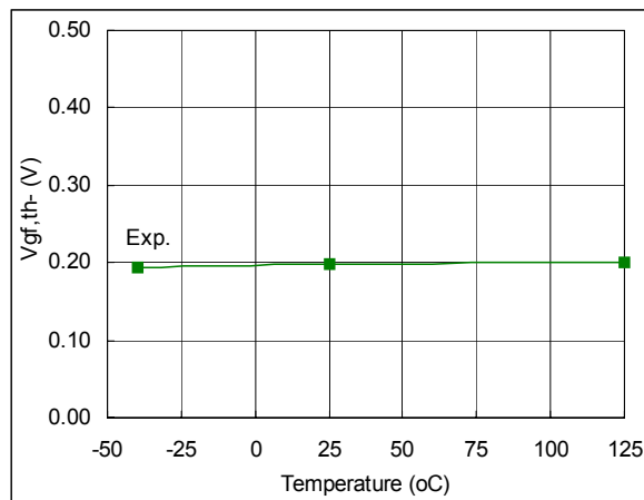
Fig. 101. GF Negative Going Threshold vs. Temperature
