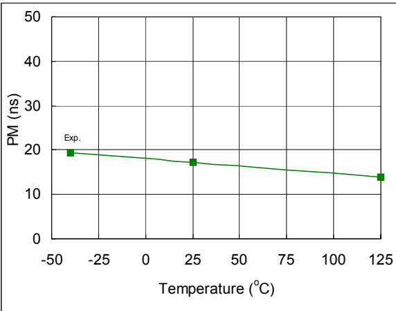
Fig. 65. Pulse Width Distortion vs. Temperature
