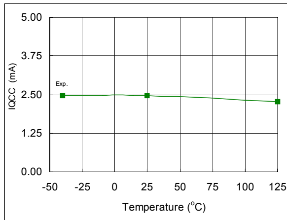
Fig. 48. Quiescent V CC Supply Current vs. Temperature
