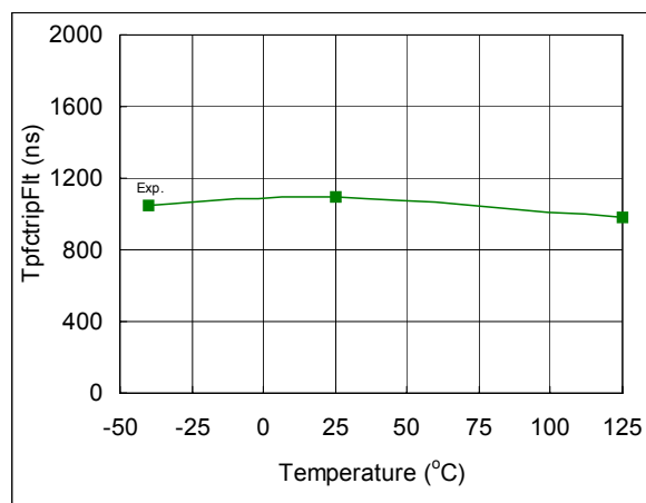
Fig. 72. PFC TRIP to Fault Time vs. Temperature
