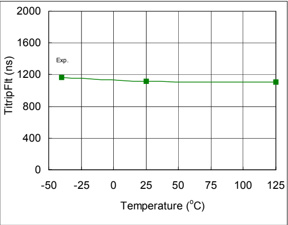
Fig. 67. ITRIP to Fault Time vs. Temperature
