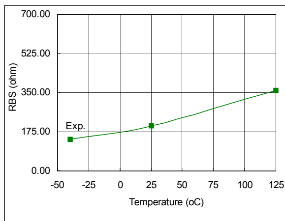
Fig. 114. R_{on} Internal Bootstrap Diode vs. Temperature
