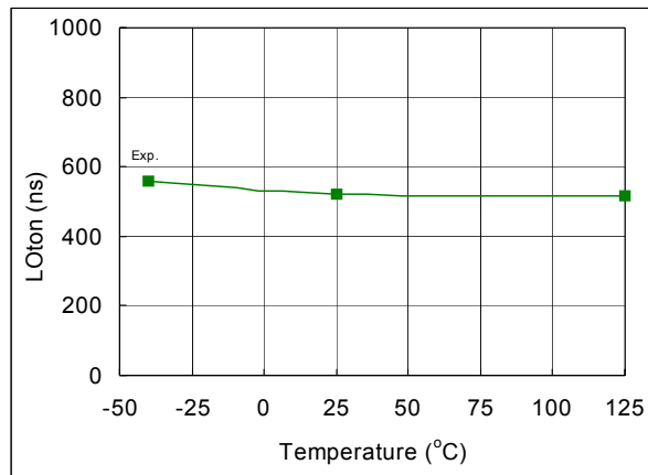
Fig. 50. Turn-On Propagation Delay vs. Temperature
