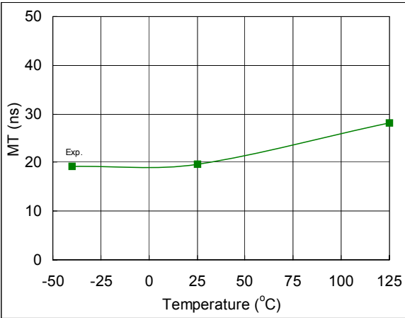
Fig. 63. Ton, Off Matching Time vs. Temperature
