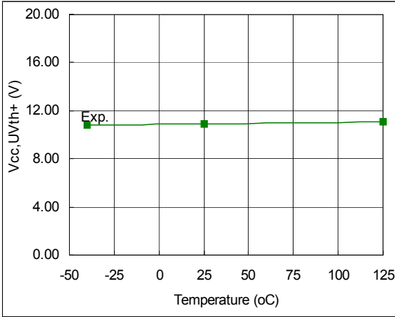
Fig. 105. V CC Supply Undervoltage Positive Going Threshold vs. Temperature
