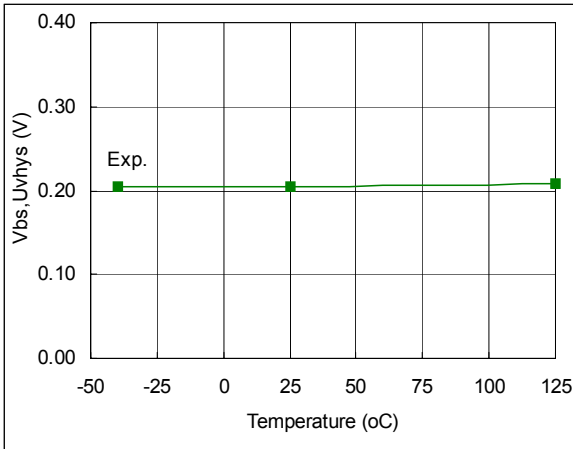
Fig. 107. V BS Supply Undervoltage Hysteresis vs. Temperature
