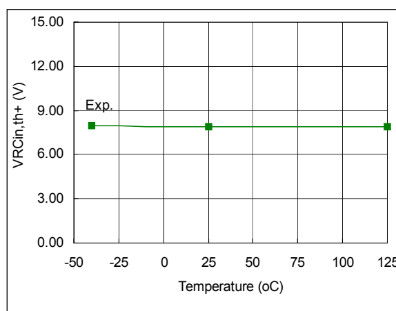
Fig. 103. RCIN Positive Going Threshold vs. Temperature
