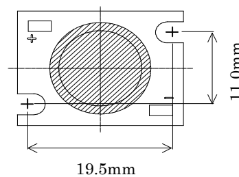
Recommended installation screw pitch
