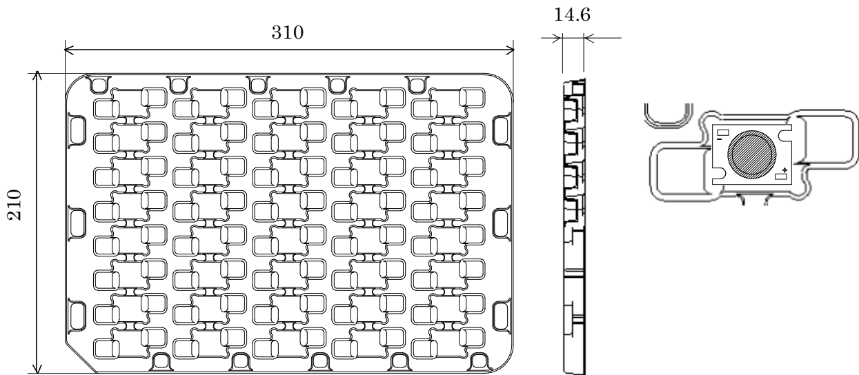
Product 40pcs/tray
