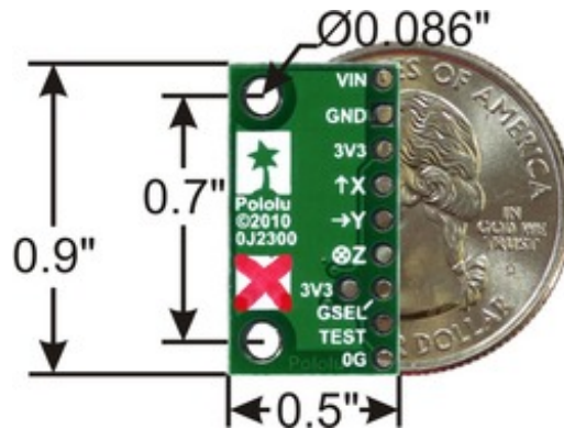
MMA7341LC 3-axis accelerometer with voltage regulator, bottom view with dimensions.
