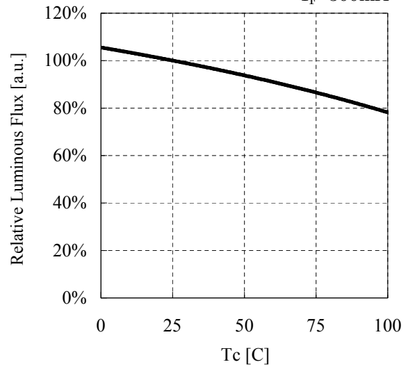
• Case Temperature vs. Relative Luminous Flux I_F=300\text{mA}
