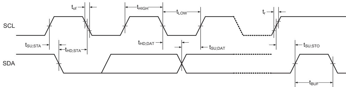
Figure 33-14. Two-wire Interface Bus Timing
