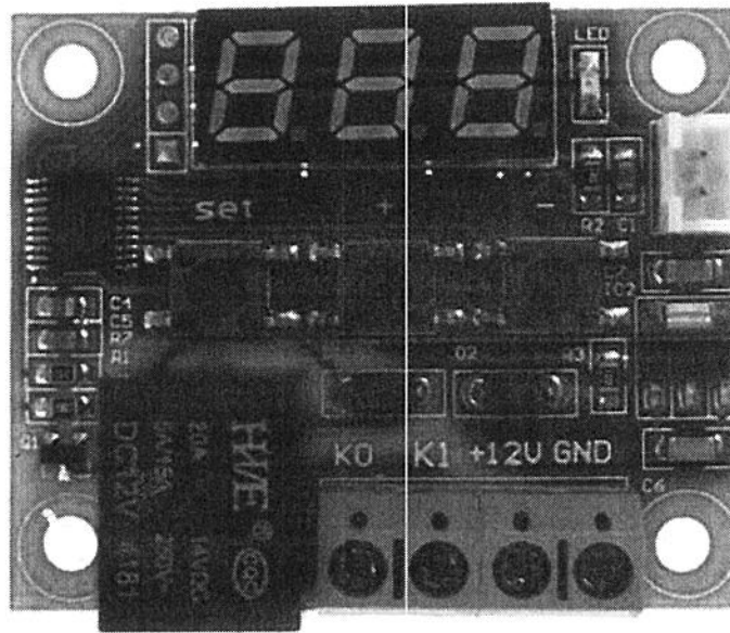
RELAY CONTACTS TO HEATER/COOLER
